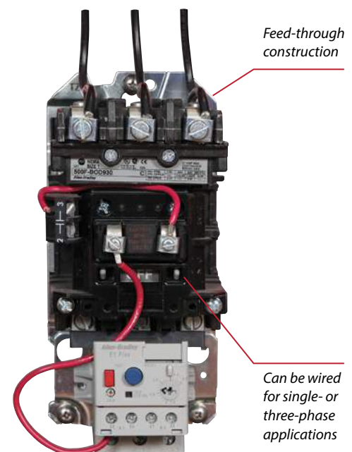
509 Open Starter
