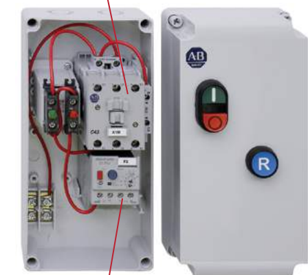
E1 Plus Electronic Overload Relay
