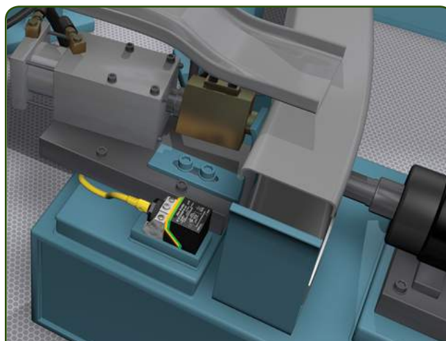
Automotive application – A VersaCube detecting the presence of a truck frame prior to initiating a weld.
